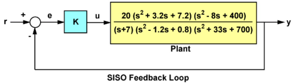
Figure 2: Feedback Loop with Multiple Phase Crossovers
